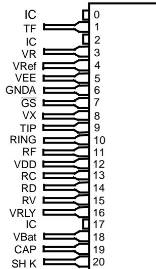
Figure 2 - Pin Connections
